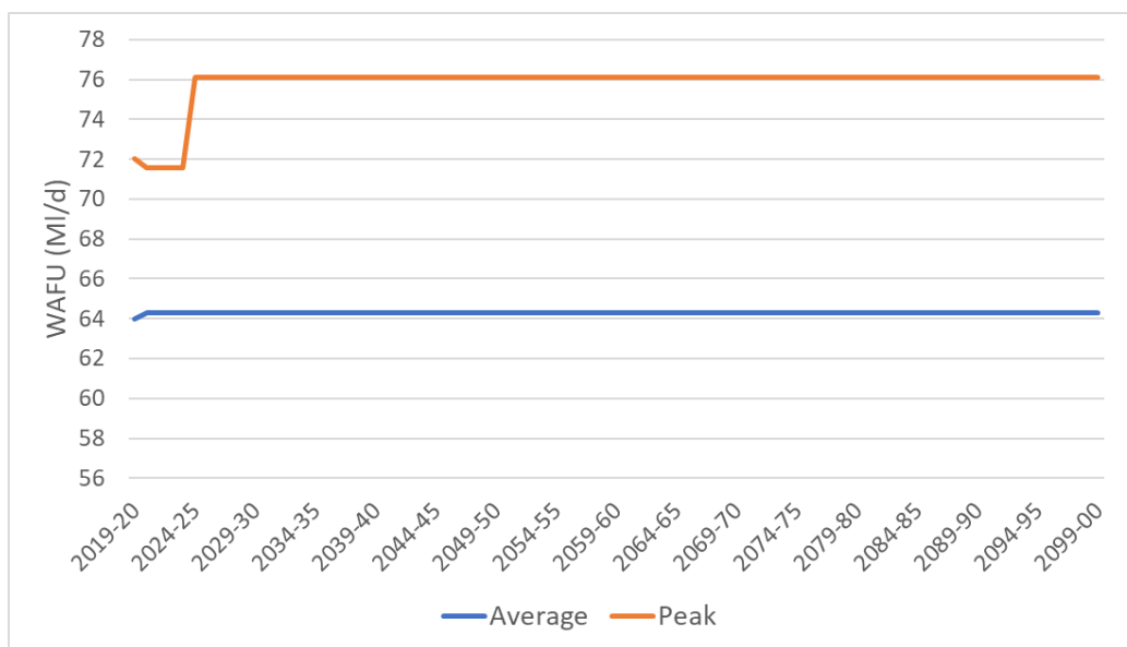
Figure 4 - 18: Guildford WAFU Forecast
