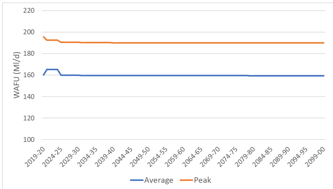
Figure 4 - 16: Slough, Wycombe & Aylesbury WAFU Forecast
