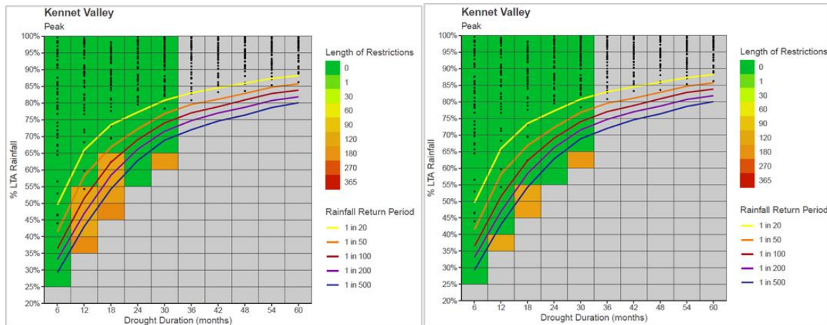
Figure 4 - 23: Kennet Valley Drought Response Surfaces, a (left), and b (right)
