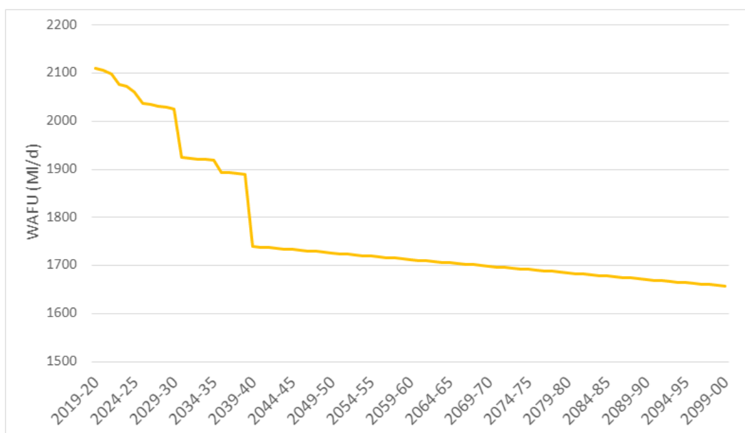
Figure 4 - 14: London DYAA WAFU Forecast
