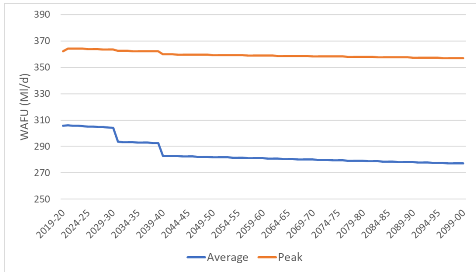
Figure 4 - 15: SWOX WAFU Forecast
