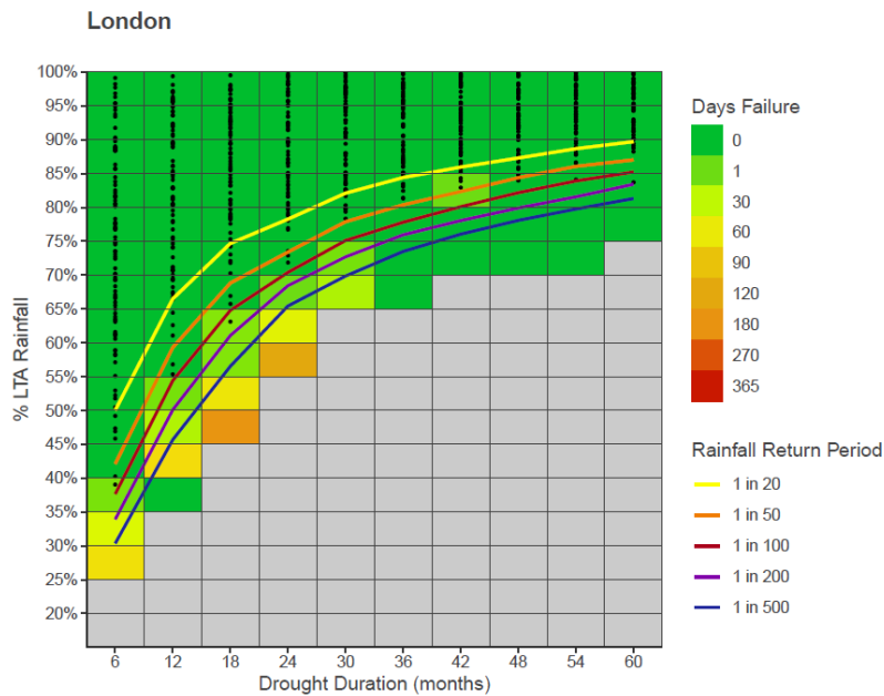
Figure 4 - 21: London Drought Response Surface
