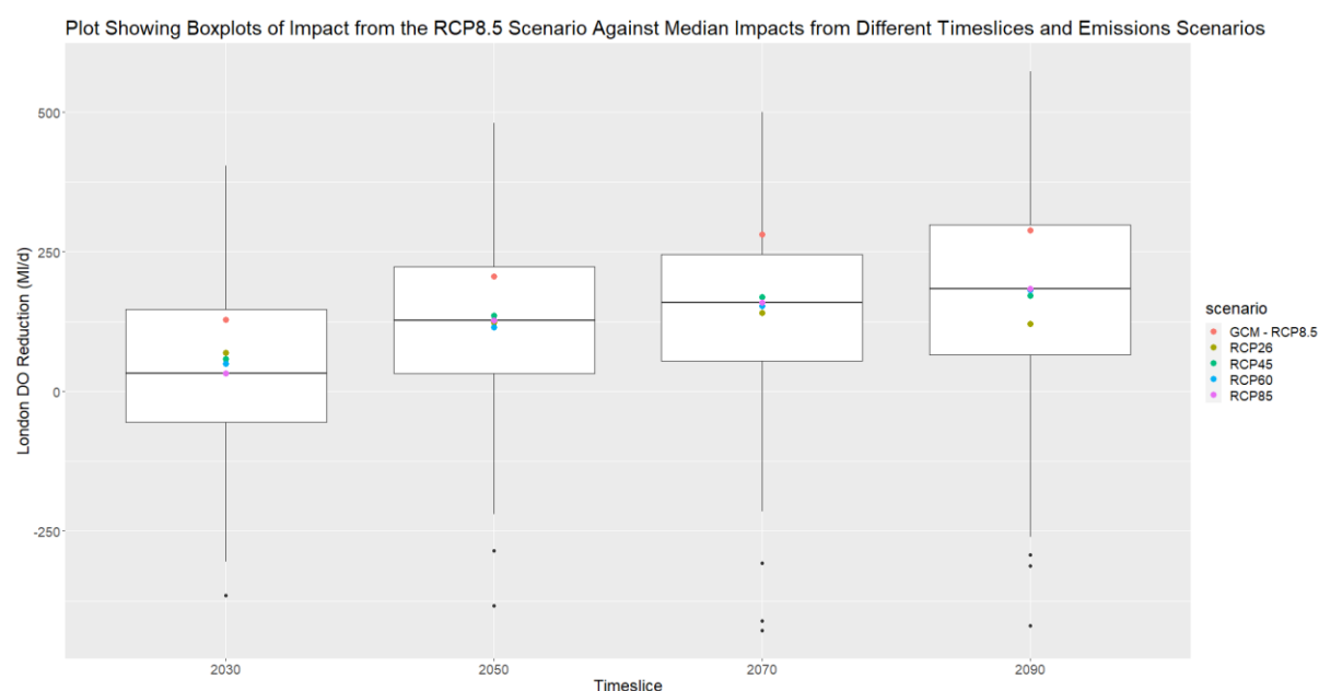
Figure 4 - 9: Overlaying Median DO Impact Projections from Different Emissions Scenarios with Boxplot of DO Impacts from a Single Emissions Scenario
