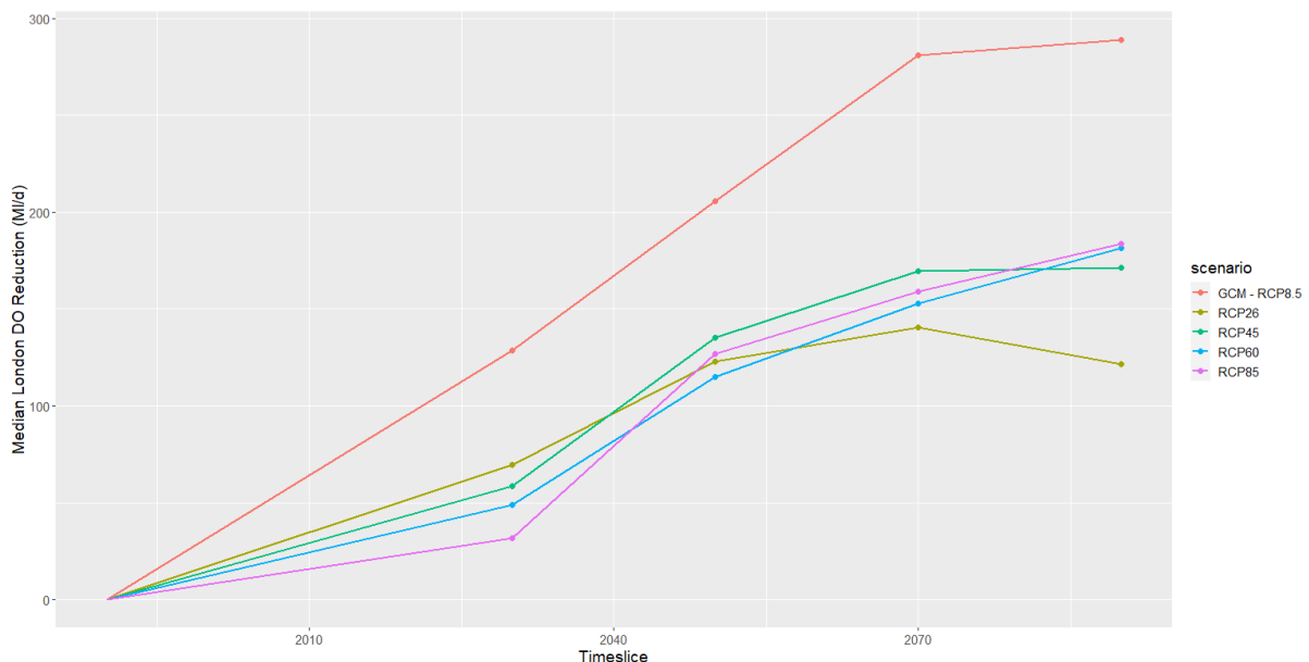
Figure 4 - 8: Median 1:500 DO Impacts from Each Combination of Timeslice and Emissions Scenario
