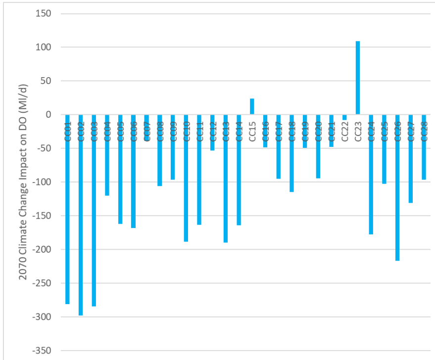
Figure 4 - 11: Impact of 28 Climate Change Projections on London DO in 2070
