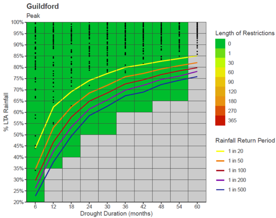
Figure 4 - 25: Guildford Drought Response Surface
