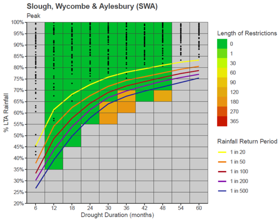
Figure 4 - 24: SWA Drought Response Surface
