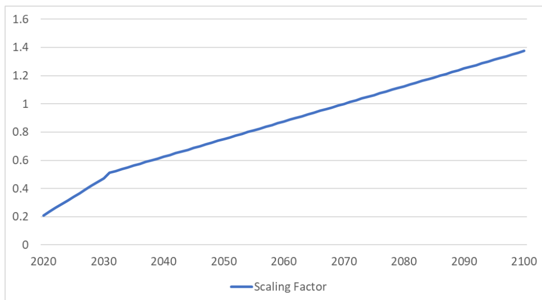
Figure 4 - 13: Climate Change Scaling Factors
