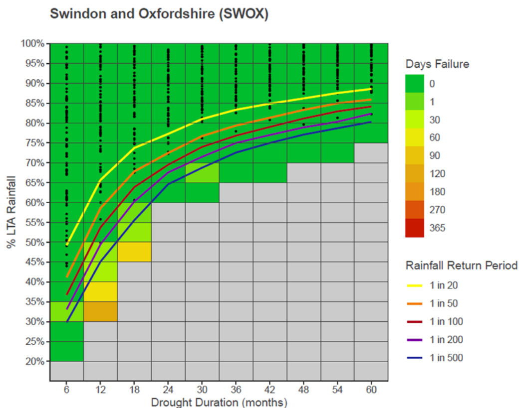
Figure 4 - 22: SWOX Drought Response Surface
