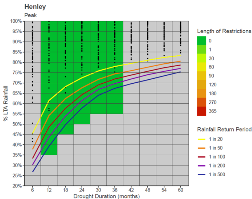
Figure 4 - 26: Henley Drought Response Surface
