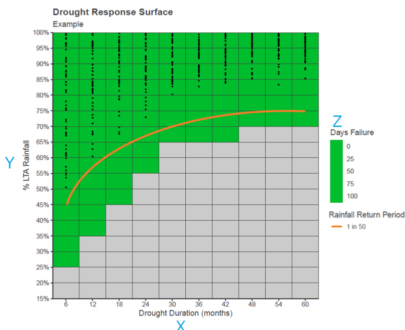
Figure 4 - 20: Example Drought Response Surface
