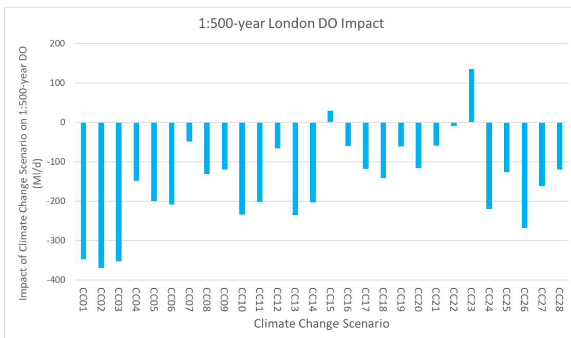
Figure 4 - 6: London DO Impact of Climate Change from 28 RCM and GCM scenarios, RCP8.5
