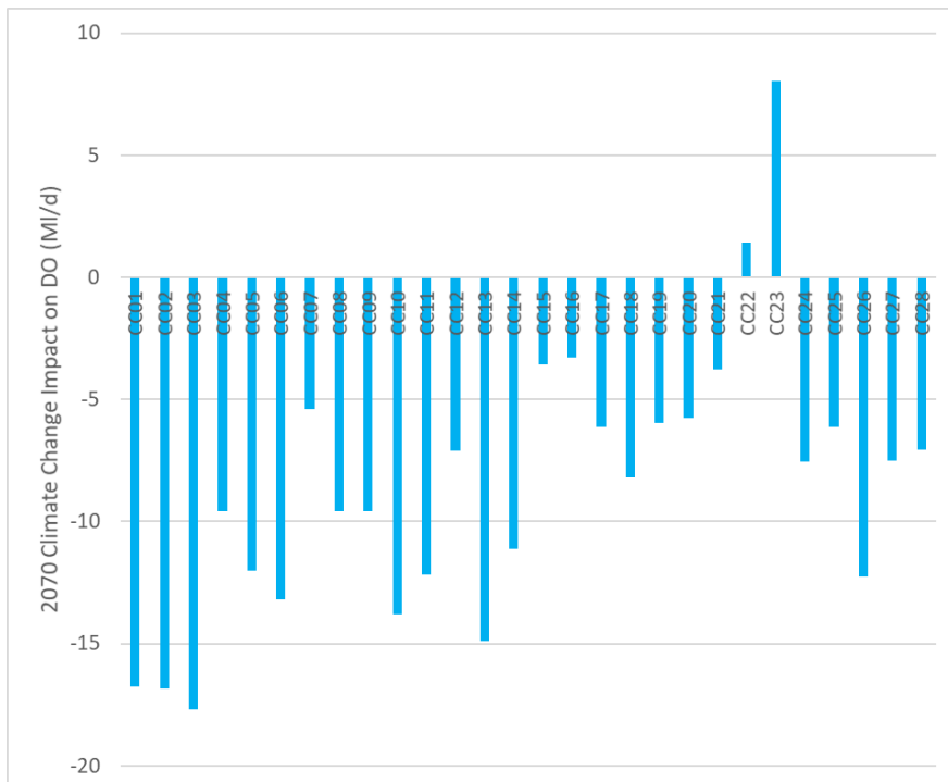
Figure 4 - 12: Impact of 28 Climate Change Projections on SWOX DYAA DO in 2070
