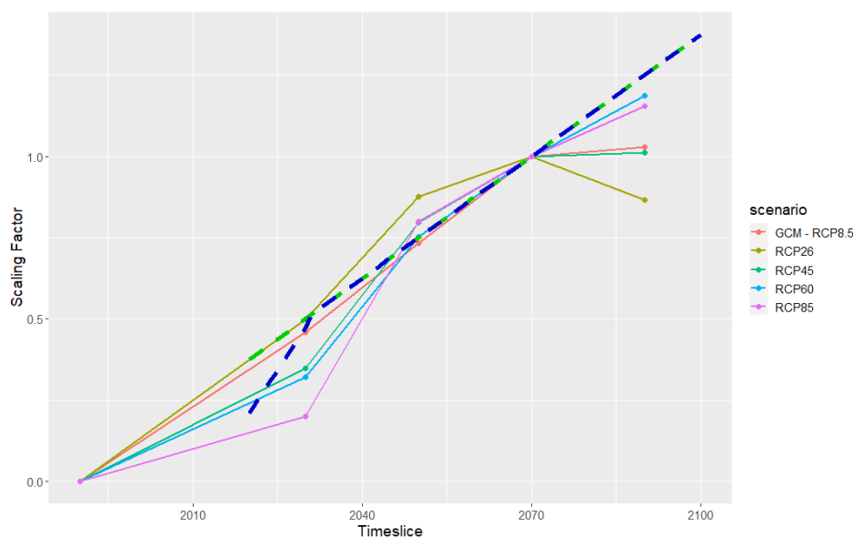
Figure 4 - 10: Scaling Factor as Calculated From Projections (Solid Lines), Compared to the 'Modified EA Standard' (Scaling linearly from 1990-2070, Green Dotted) and "Alternative EA Scaling" (Blue Dotted)
