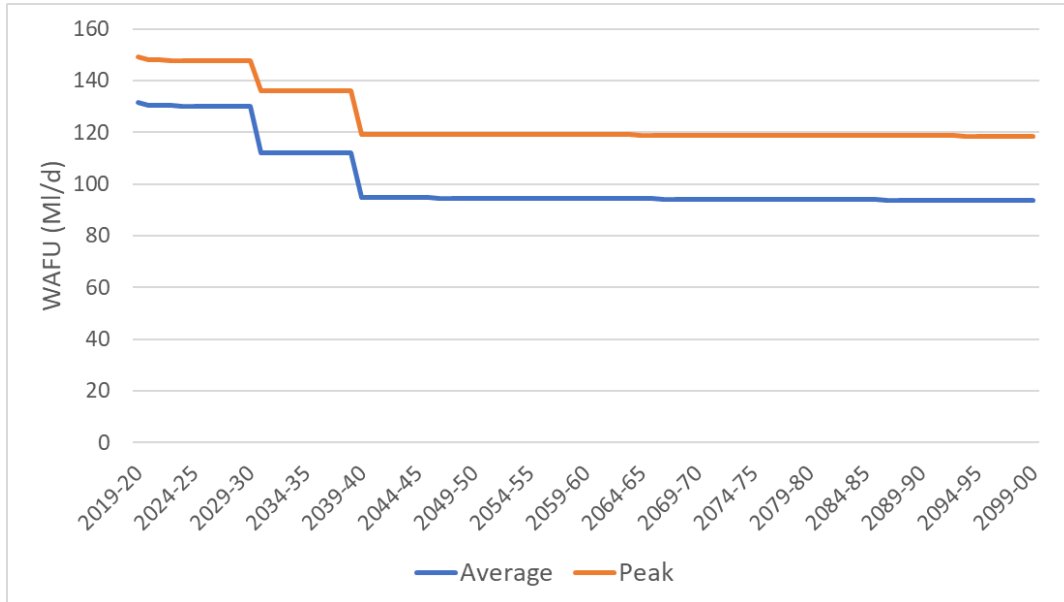
Figure 4 - 17: Kennet Valley WAFU Forecast
